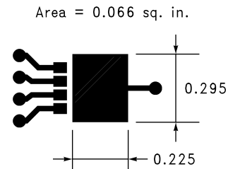
Figure 21. SCENARIO B, \theta_{JA} = 125^{\circ}\text{C/W}
